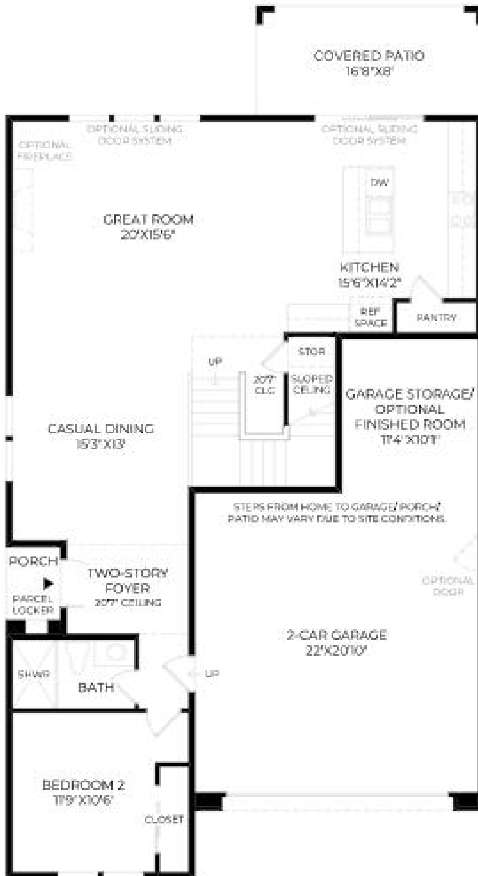
FIRST FLOOR 10' CEILING HEIGHT
