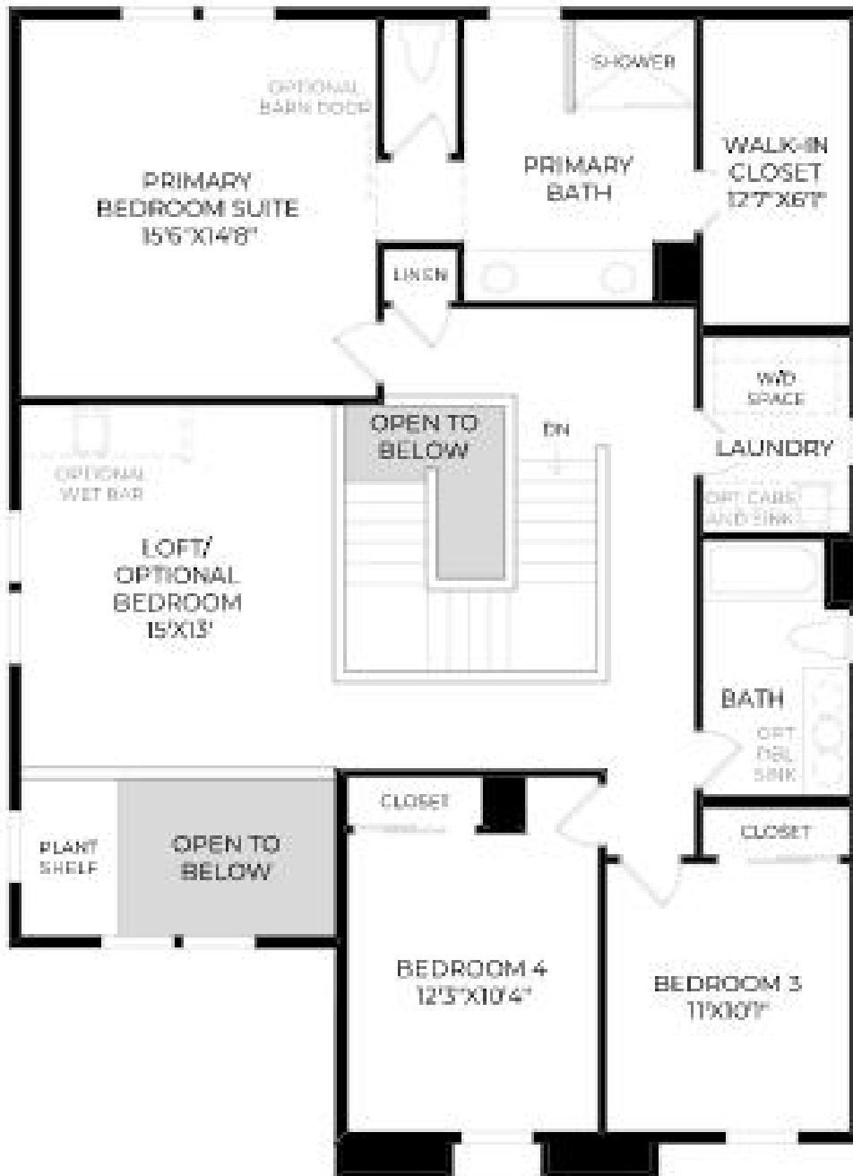
SECOND FLOOR 9' CEILING HEIGHT
