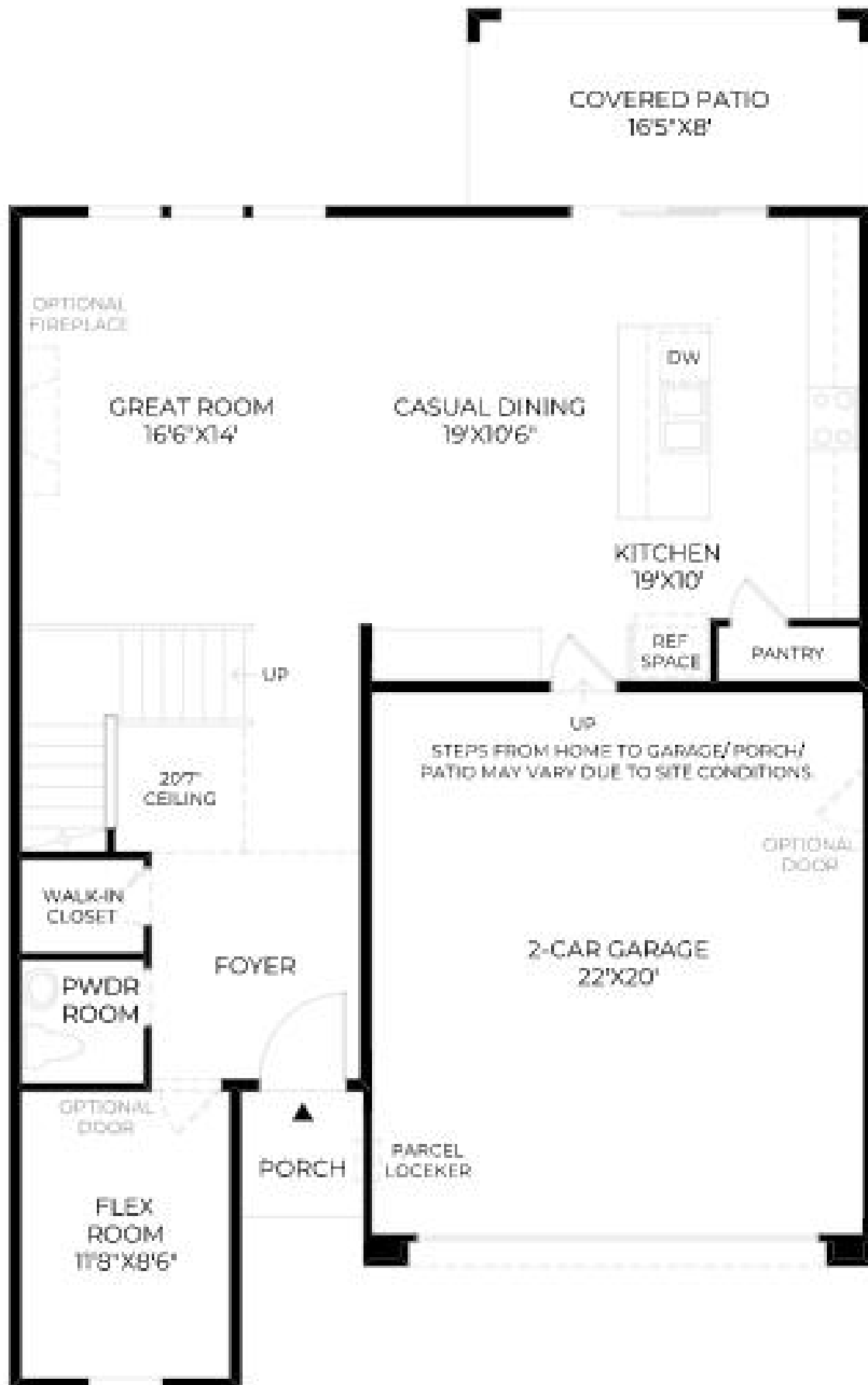
FIRST FLOOR 10' CEILING HEIGHT
