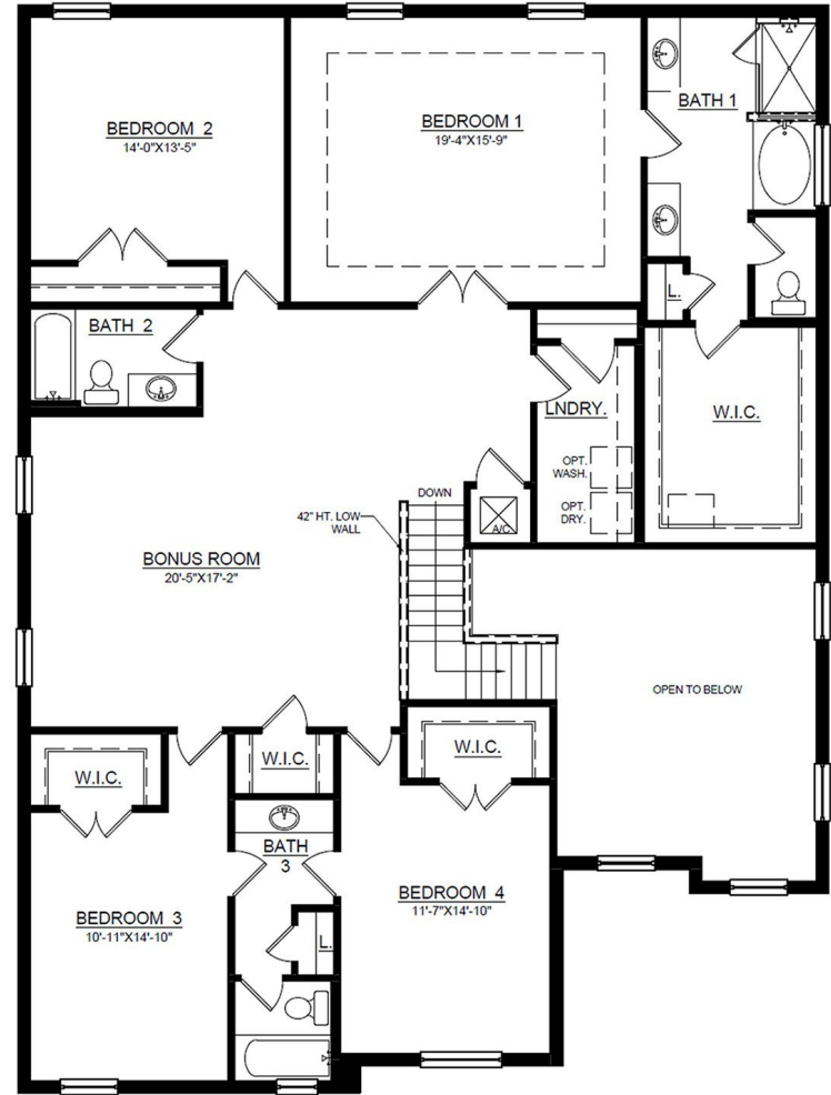
Second Floor Plan - Elevation G & H
