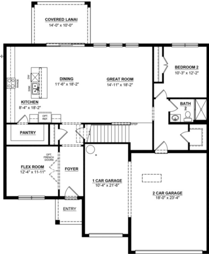
First Floor - Elevation G
