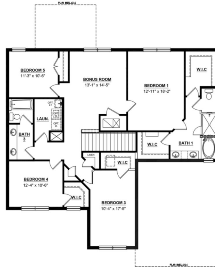
Second Floor - Elevation G & H
