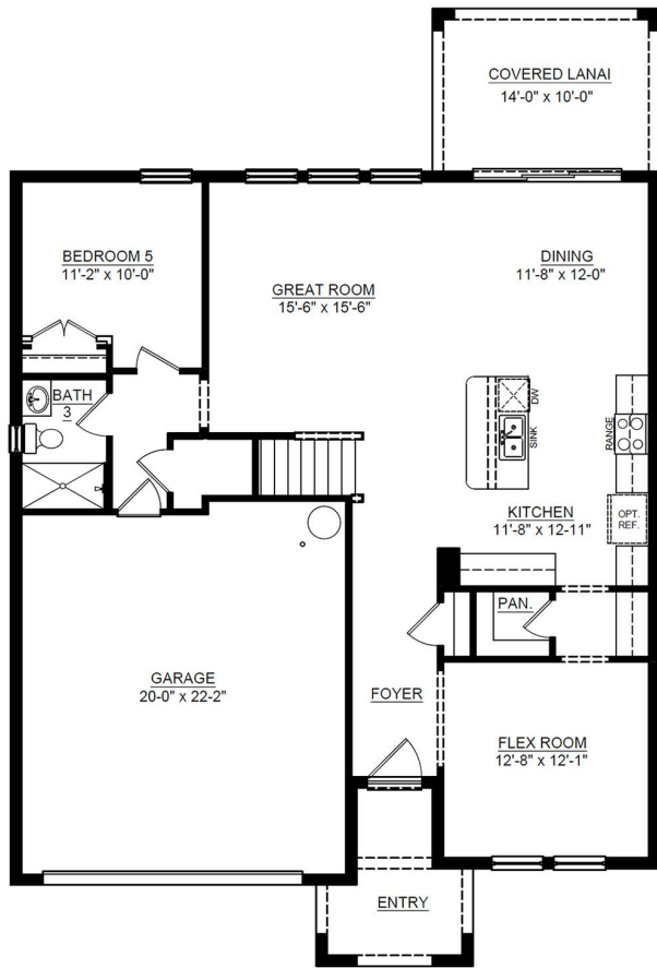
First Floor Plan - Elevation G
