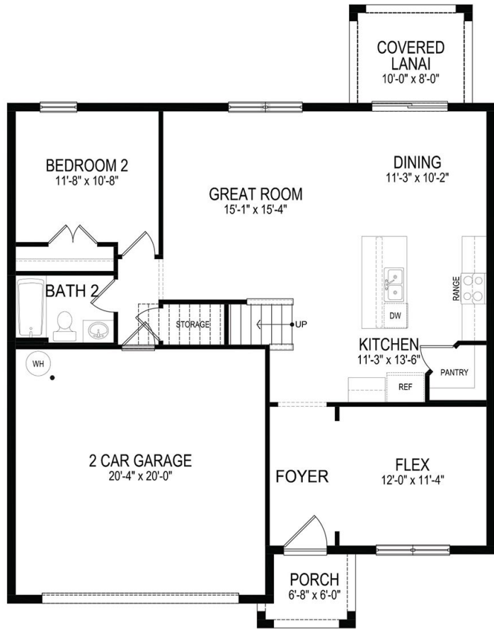
FIRST FLOOR - Elevation G & J
