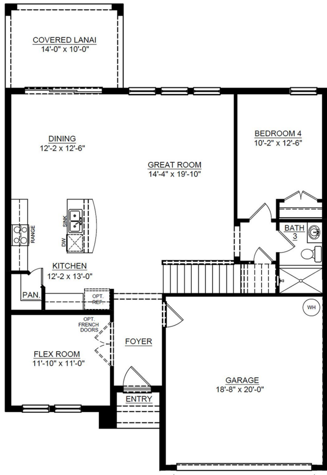
First Floor Plan - Elevation G
