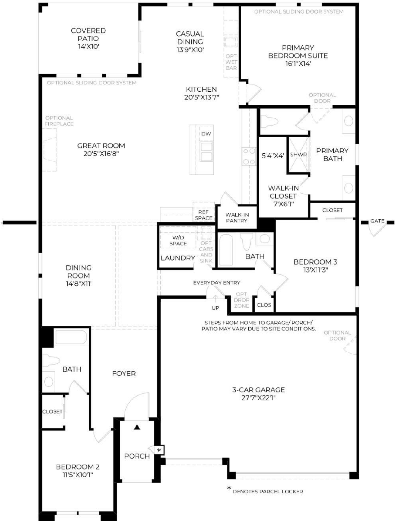
FLOOR PLAN 10' CEILING HEIGHT
