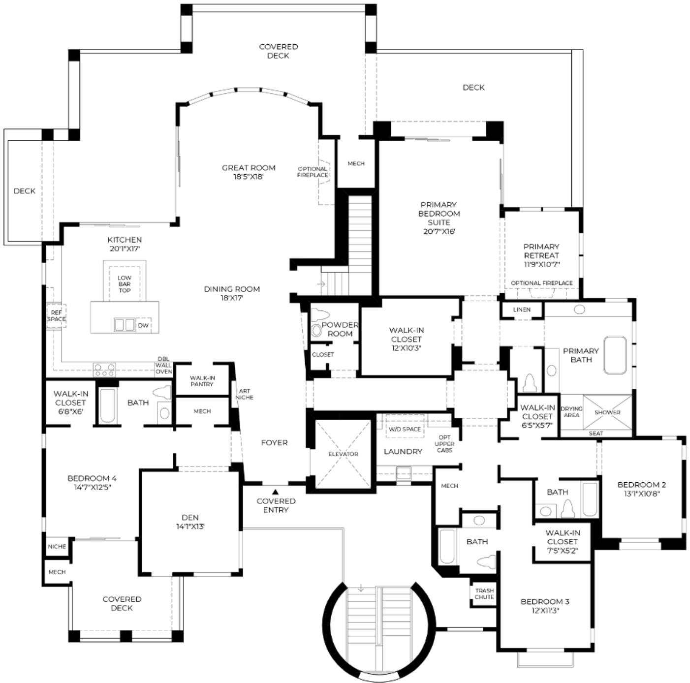
Floor Plan 10' CEILING HEIGHT
