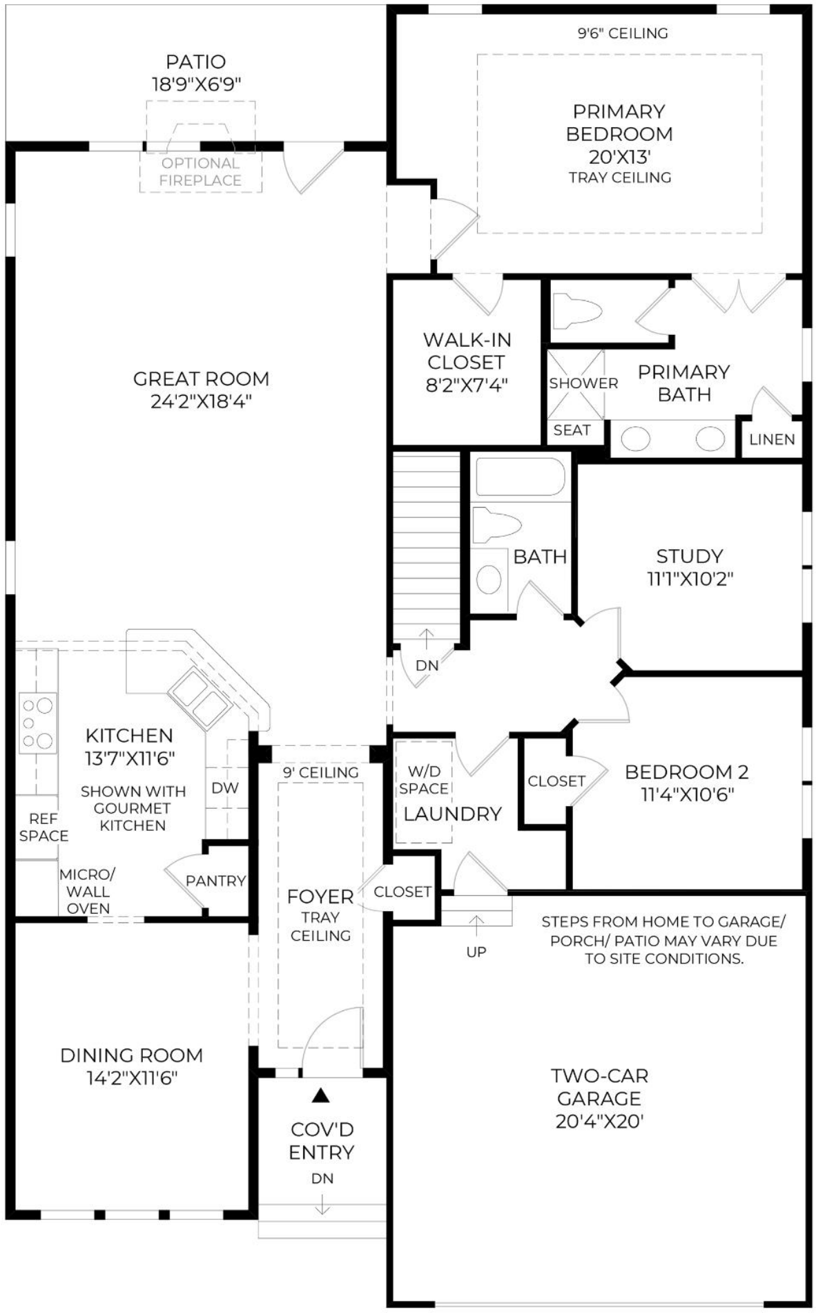
Floor Plan 10' CEILING HEIGHT
