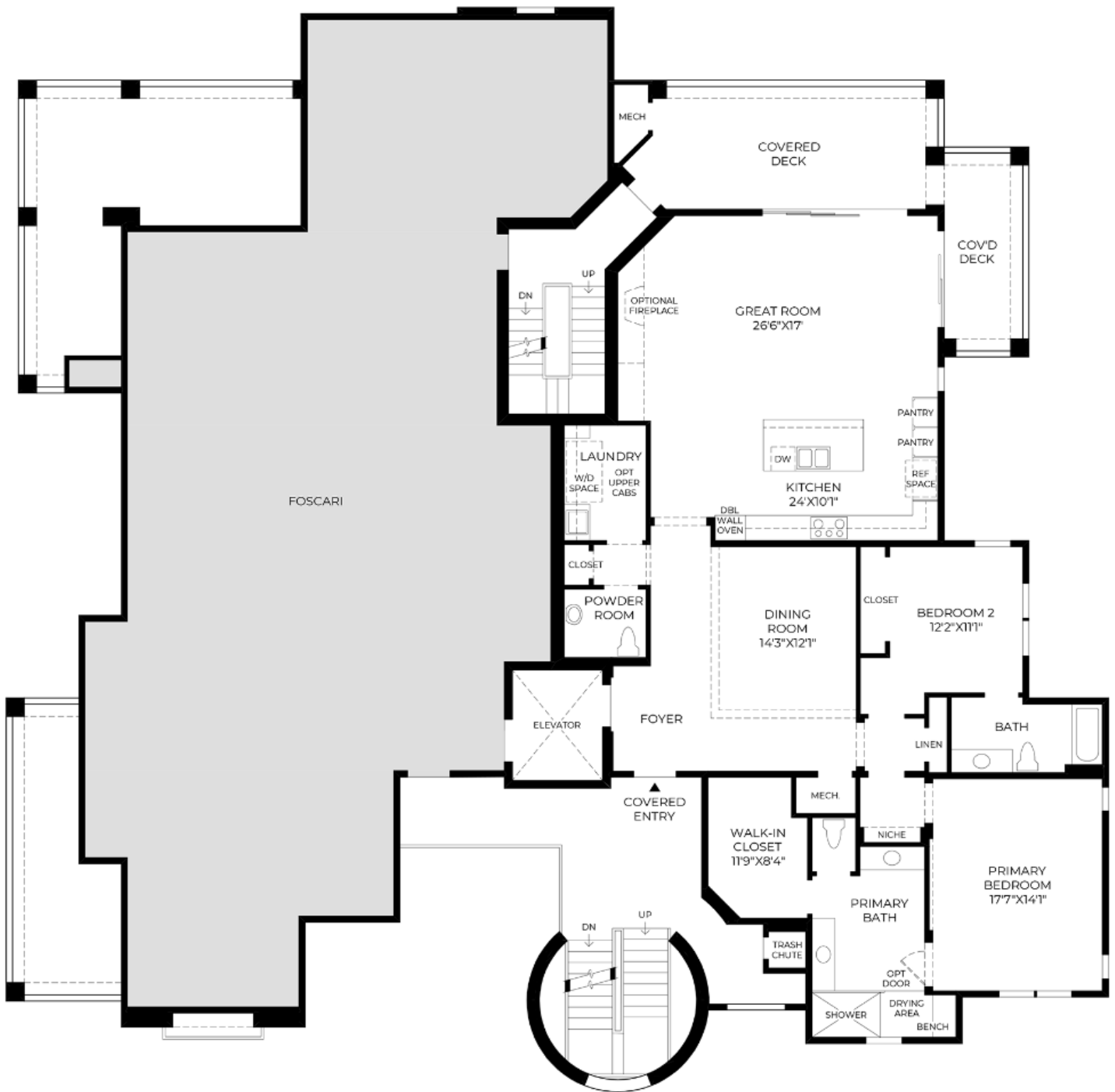
Floor Plan 10' CEILING HEIGHT
