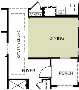
OPT. FORMAL DINING ILO FLEX
