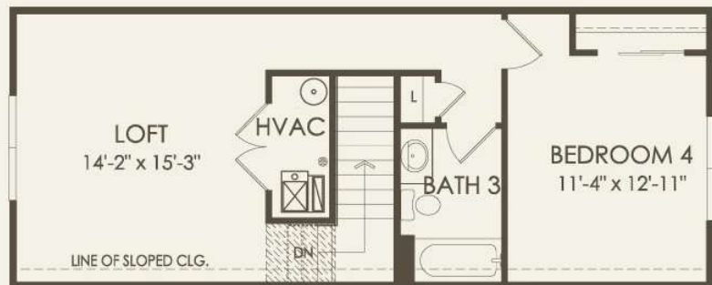
Opt. Second Floor Plan - Slab Foundation
