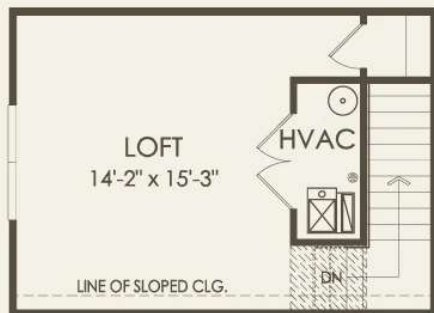
Opt. Loft - Slab foundation
