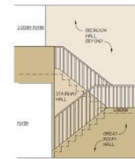
OPTIONAL OPEN STAIRWAY ELEVATION
